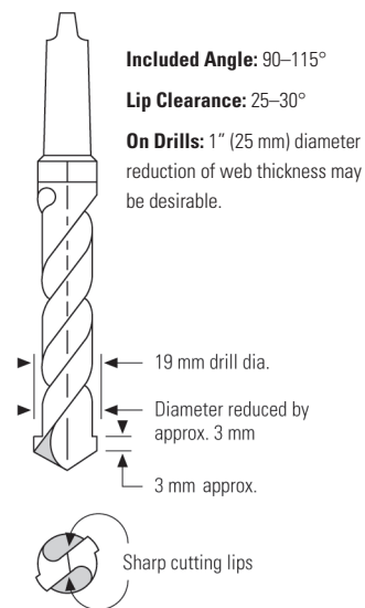
Figure 2: Modified Drill for Vespel® Shapes
