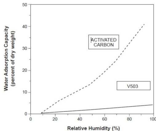
Figure 1: Moisture Uptake AmberSorb™ V503 Polymeric Adsorbent vs. Activated Carbon
