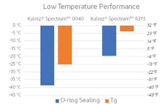
Low temperature static sealing (DuPont Proprietary test method)
