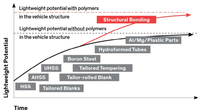
Figure 1 - New weight-reduction potential with structural adhesives.
