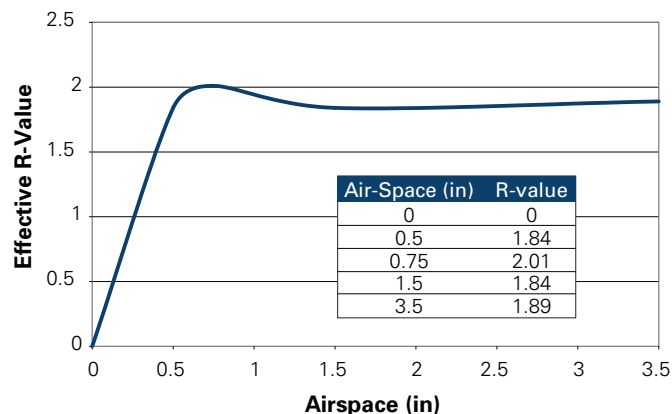
Figure 1. Calculated R-value per ASHRAE Handbook of Fundamentals
