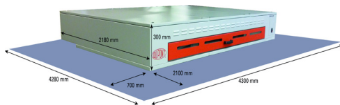
Floor Plan
