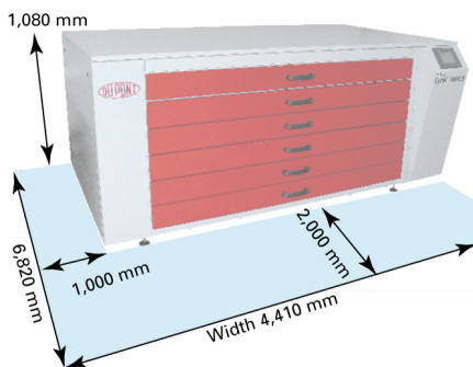
Floor Plan
