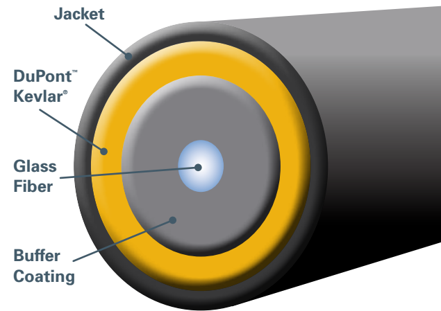
Cross-sectional view of a single fiber optical cable shows the tight buffered fiber completely covered by DuPont™ Kevlar® K29 AP 600 denier yarn.
