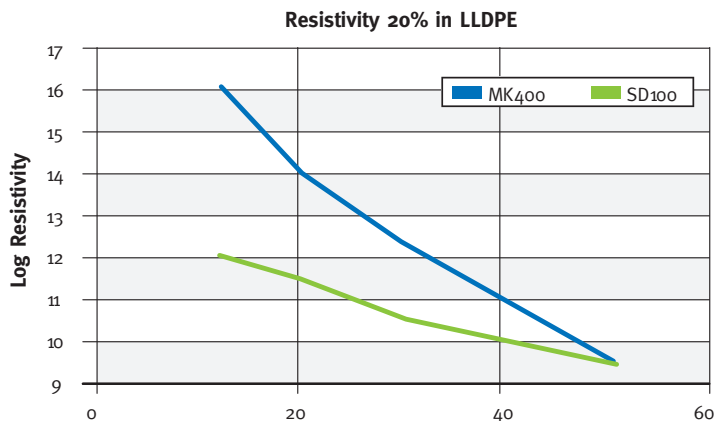
Chart 1: DuPont™ Entira™ Antistat performance at different humidity
