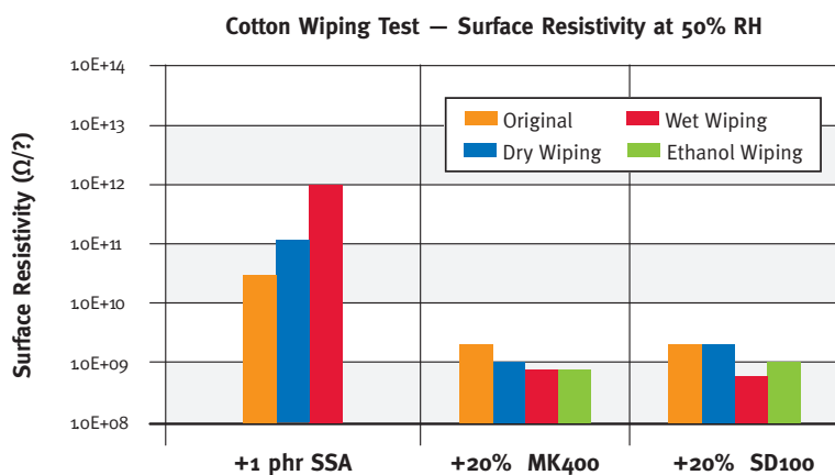
Chart 2: DuPont™ Entira™ Antistat provides lower surface resistivity than typical Surface Active Agents (SAA)
