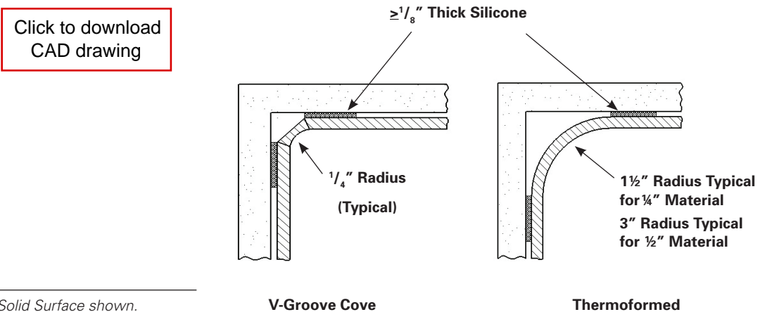
Figure 6 Hardseamed Corners
