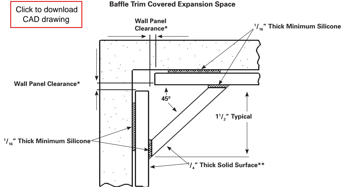
Figure 7c Baffle Trim Covered Expansion Space
