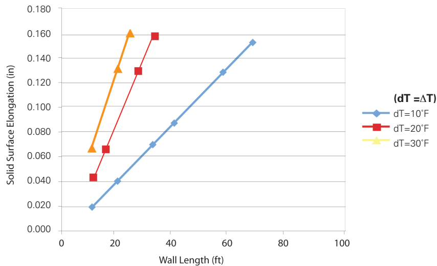
Figure 4 Wall Expansion and Contraction
