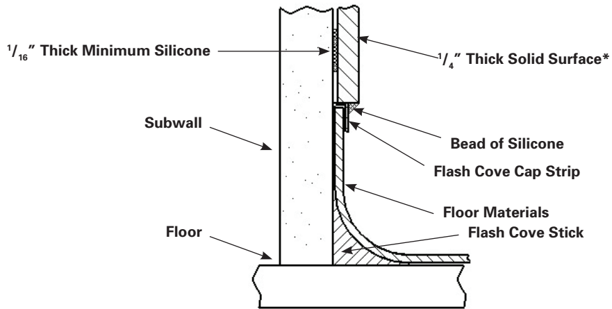
Floor Detail Alternative with Flash Cove
