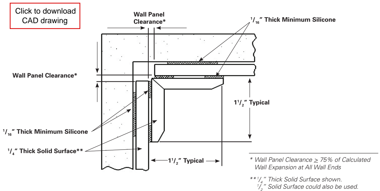
Figure 7a V-Groove Trim Covered Expansion Space
