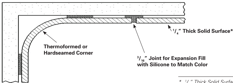
Figure 10 Silicone Soft Seams
