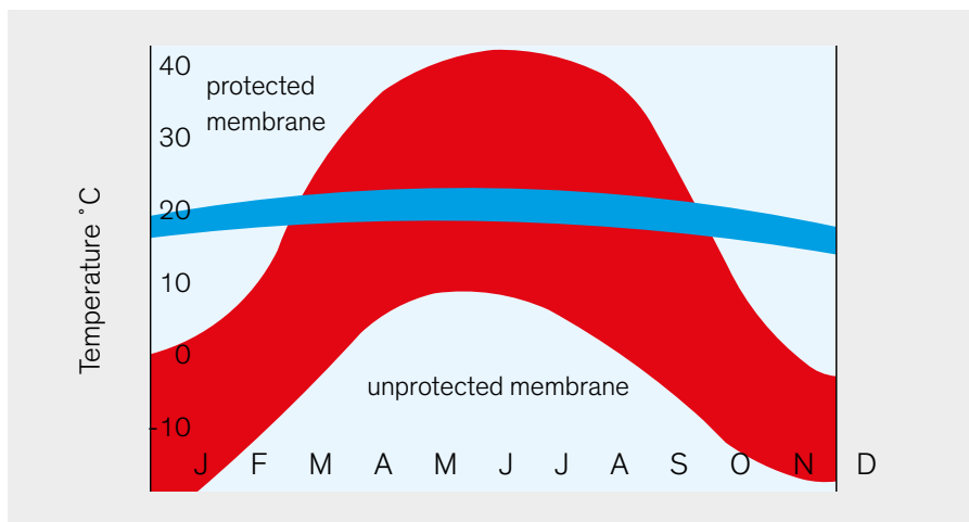
Figure 1: Temperature fluctuations in an unprotected roof covering compared with those in one protected by XENERGY™
