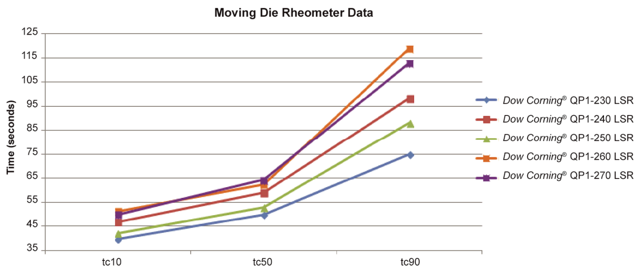
Figure 1: Moving Die Rheometry Data 1
