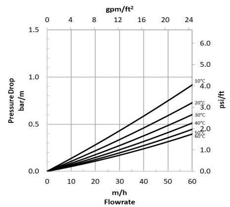
Figure 2: Pressure Drop
