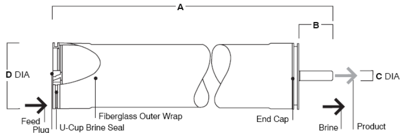
Figure 1: Element Dimensions
