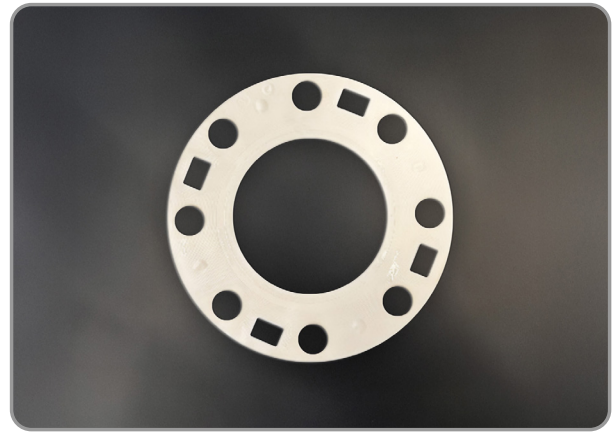
Tedlar® gasket extracted from electrolyzer after 5000+ hrs accelerated testing maintaining physical integrity and showing no deformation.
