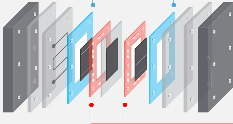
Typical PEM electrolyzer cross-section showing the gasket and the subgasket
