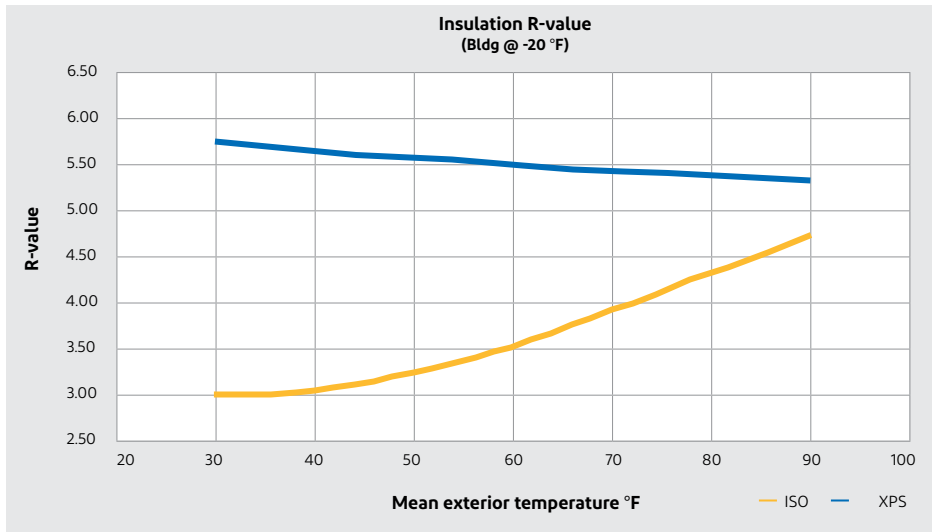
Figure 3. Effective R of Roofing ISO and DuPont™ Styrofoam™ for Building Maintained at -20°F
