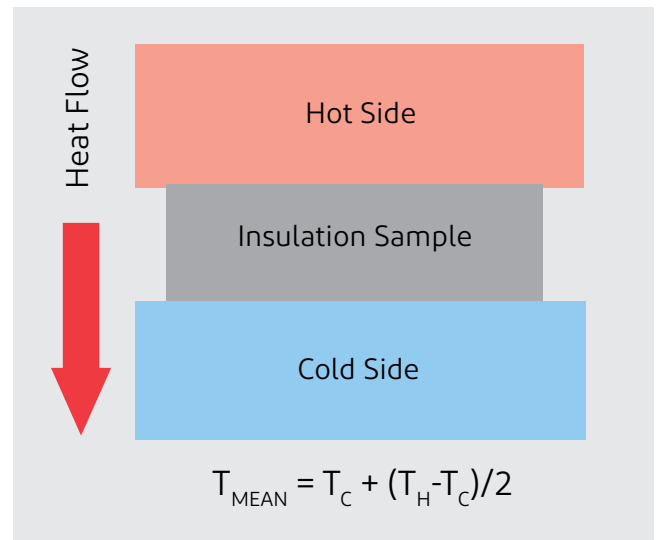
Figure 1. Thermal Resistance and Mean Temperature
