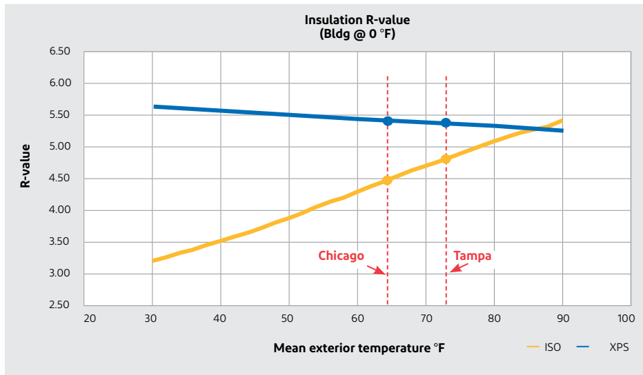
Figure 4. Effective R of Roofing ISO and DuPont™ Styrofoam™ for Building Maintained at 0°F
