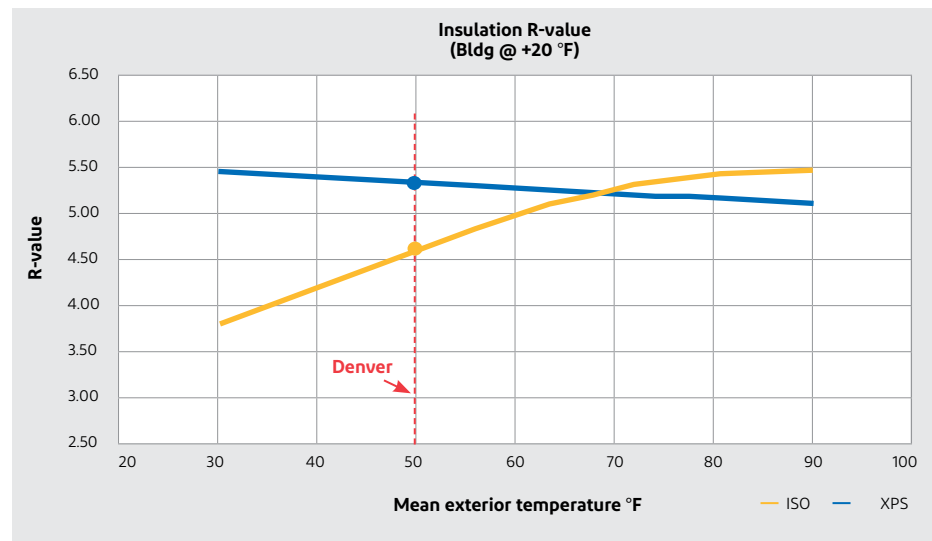
Figure 5. Effective R of Roofing ISO and DuPont™ Styrofoam™ for Building Maintained at +20°F
