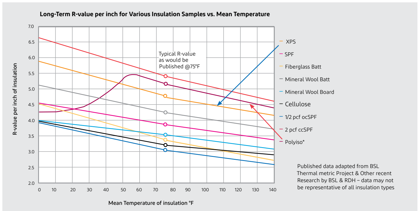
Figure 2. Thermal Resistance versus Insulation Mean Temperature
