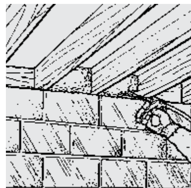
Figure 10: Insulating sill plate/rim joists (maximum 2" [50 mm] thickness)
