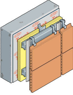
Fig. 7 Masonry * Rainscreen cladding
