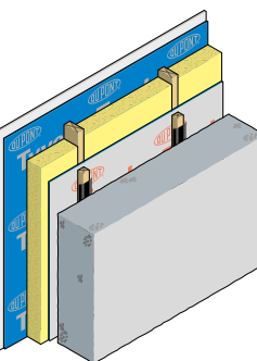
Fig. 6 Masonry * Internal insulation upgrade
