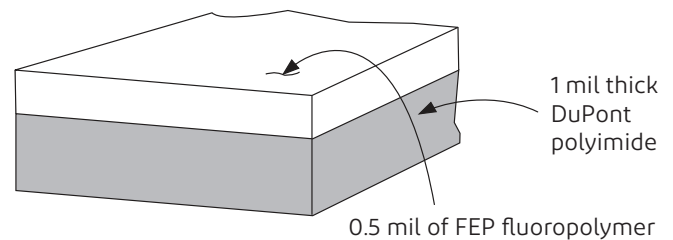
Figure 1. Construction of Kapton® 150FWN019
