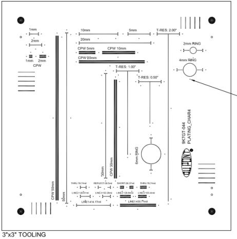
Fig. 2 High frequency test pattern.
