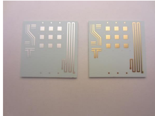
Fig. 1 Standard adhesion test pattern.
