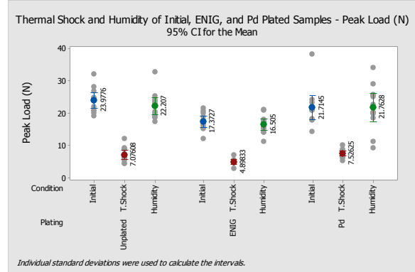
Fig. 3 Thermal shock & humidity adhesion peak load (N).
