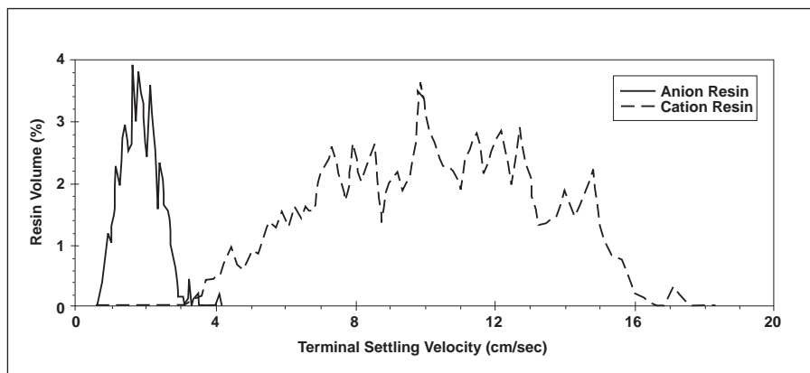
Figure 2. Terminal Settling Velocity for Conventional Resins with a Gaussian Particle Size Distribution
