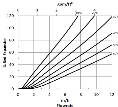
Figure 1: Backwash Expansion
