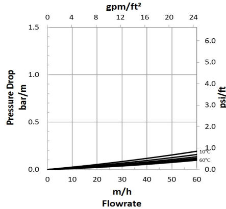
Figure 1a: Pressure Drop Temperature = 10 – 60°C (50 – 140°F)
