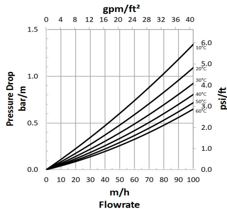
Figure 1: Pressure Drop
