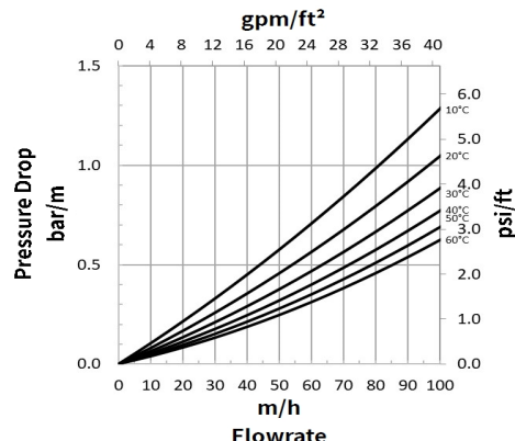
Figure 2: Pressure Drop
