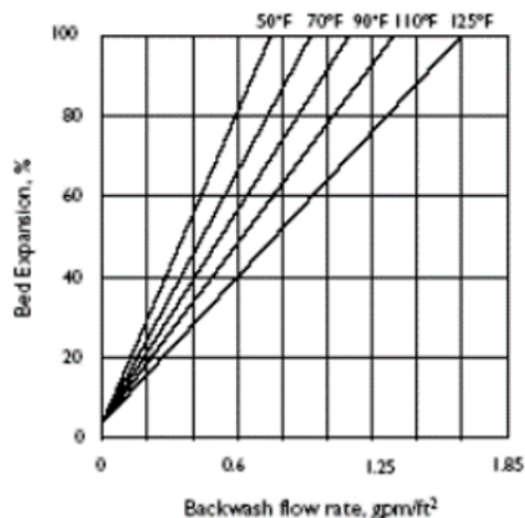
Figure 1: Backwash Expansion
