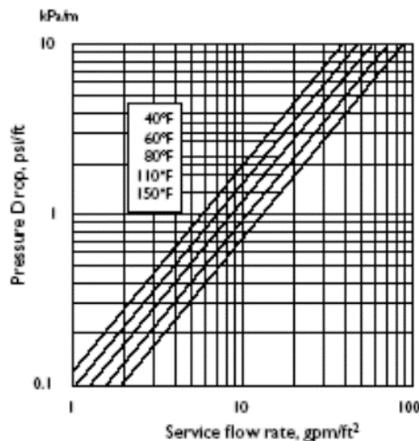
Figure 2: Pressure Drop
