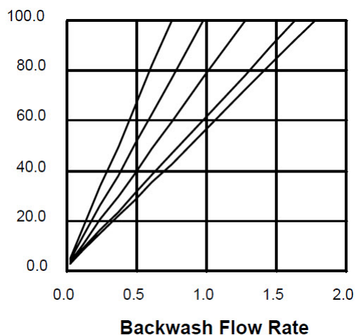
Figure 1: Backwash Expansion
