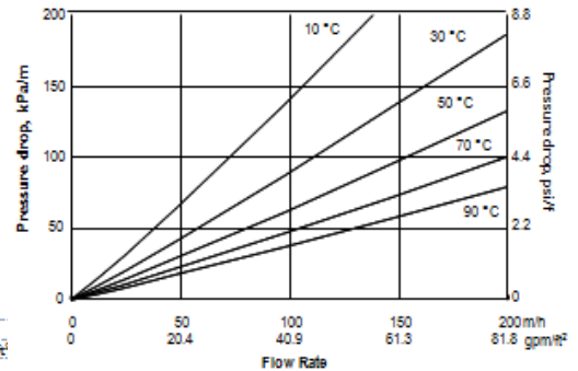
Figure 2: Pressure Drop
