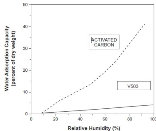
Figure 1: Moisture Uptake
