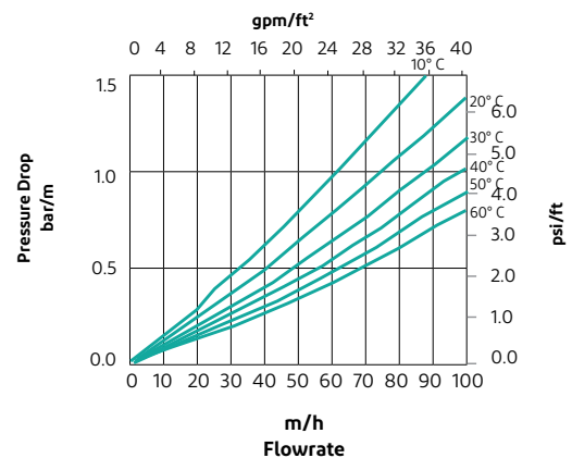
Figure 2. Pressure Drop Temperature = 10 – 60°C (50 – 140°F)
