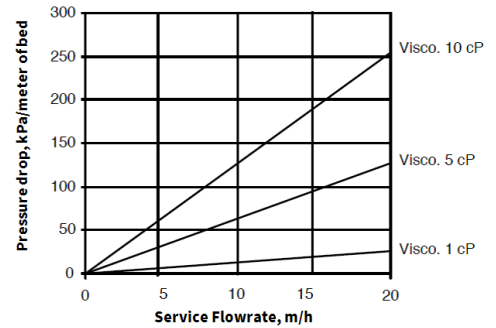
Figure 2: Pressure Drop Viscosity = 1 – 10 cP
