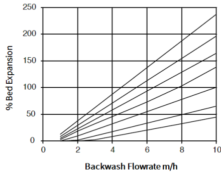
Figure 1: Backwash Expansion Temperature = 5 – 60°C (41 – 140°F)
