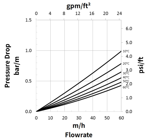
Figure 2: Pressure Drop Temperature = 10 – 60°C (50 – 140°F)
