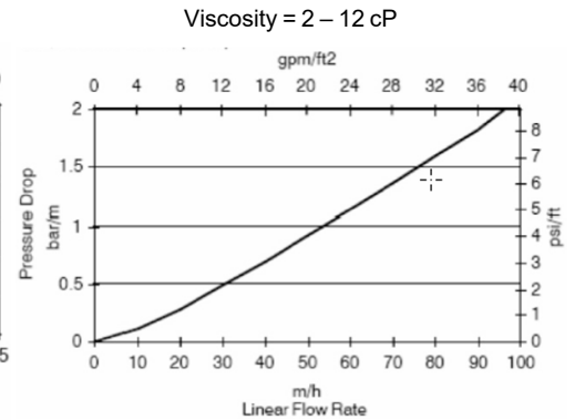
Figure 2: Pressure Drop
