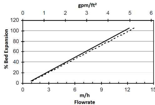
Figure 1: Backwash Expansion
