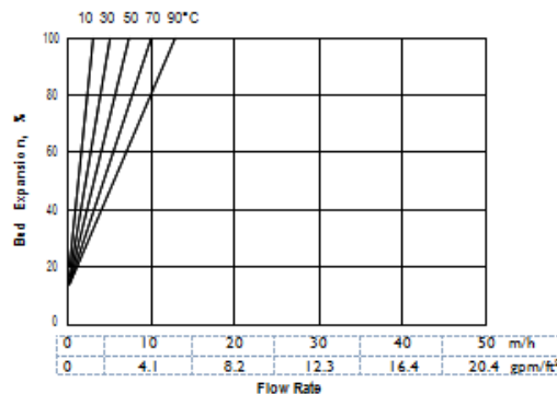
Figure 1: Backwash Expansion
