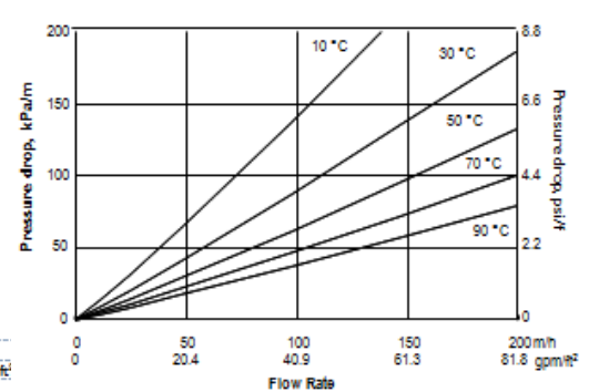
Figure 2: Pressure Drop
