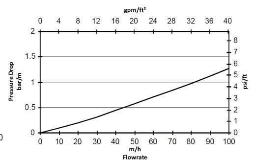
Figure 2: Pressure Drop
